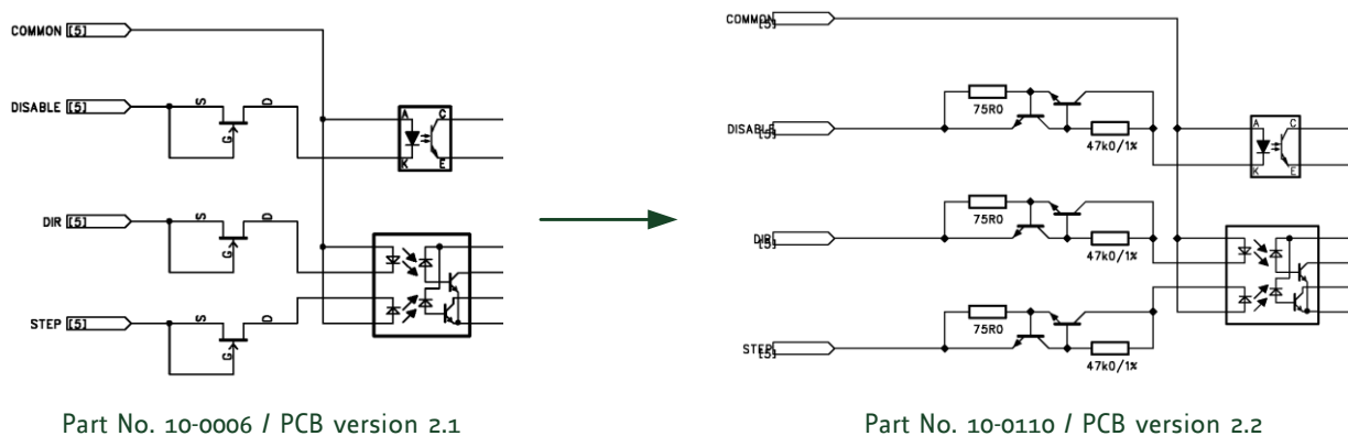
Figure 2.1: new input circuit for opto-couplers since PCB version 2.2
