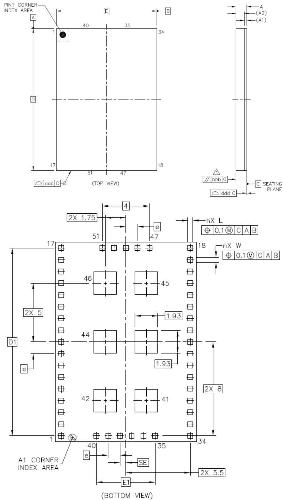
Figure 2: LGA51 package outline drawings
