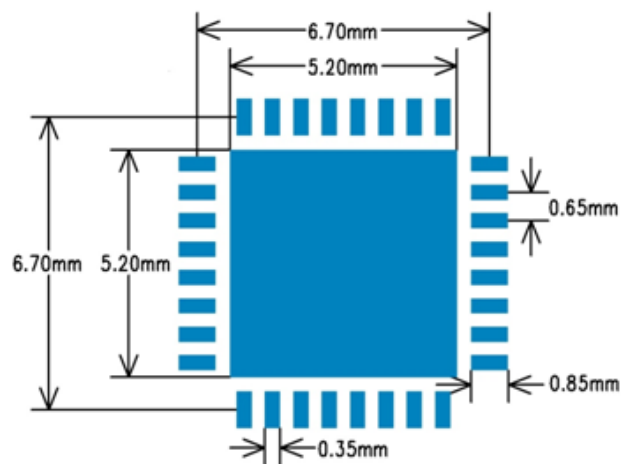
Figure 3: QFN32 (7x7mm) example land patterns (unit: mm)
