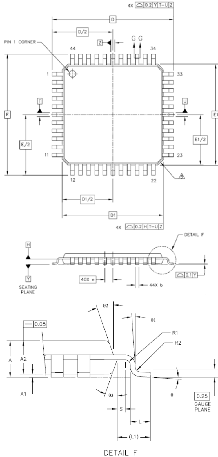
Figure 2: LQFP44 package outline drawings
