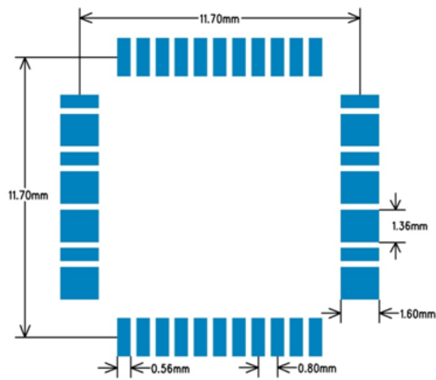
Figure 3: LQFP44 example land patterns (unit: mm)
