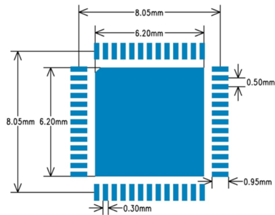
Figure 3: QFN52 (8x8mm) example land patterns (unit: mm)
