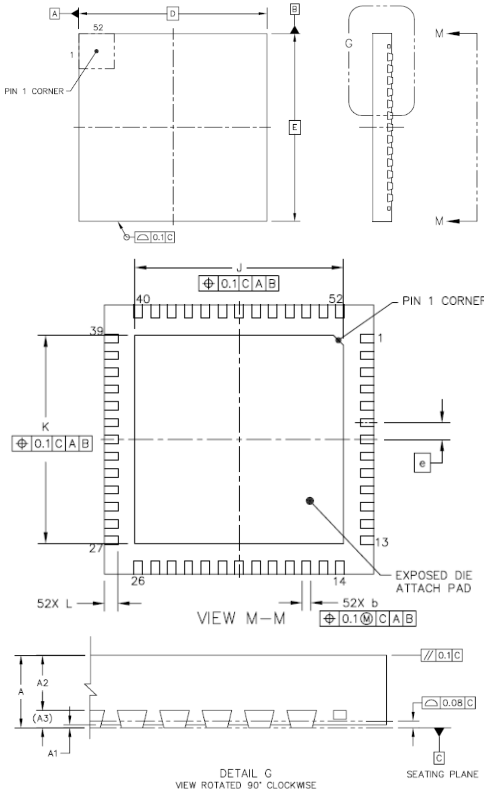
Figure 2: QFN52 (8x8mm) package outline drawings
