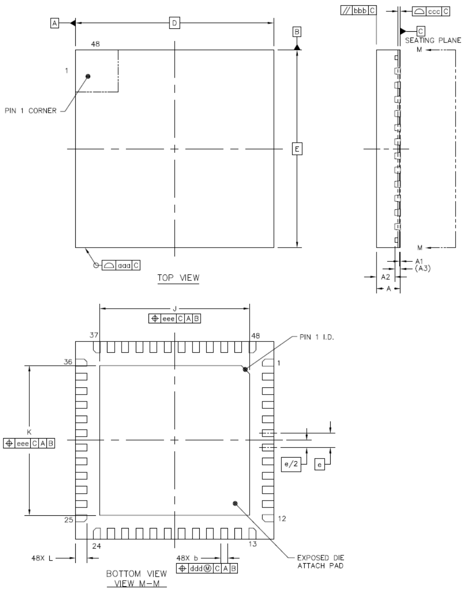
Figure 2: QFN48 (7x7mm) package outline drawings
