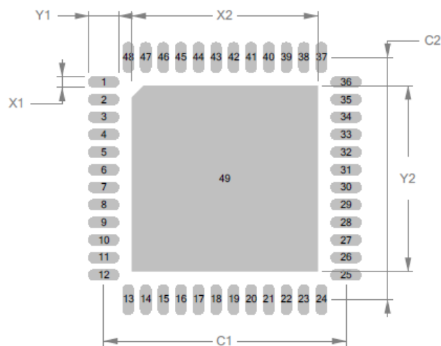
Figure 3: QFN48 (7x7mm) example land patterns (unit: mm)
