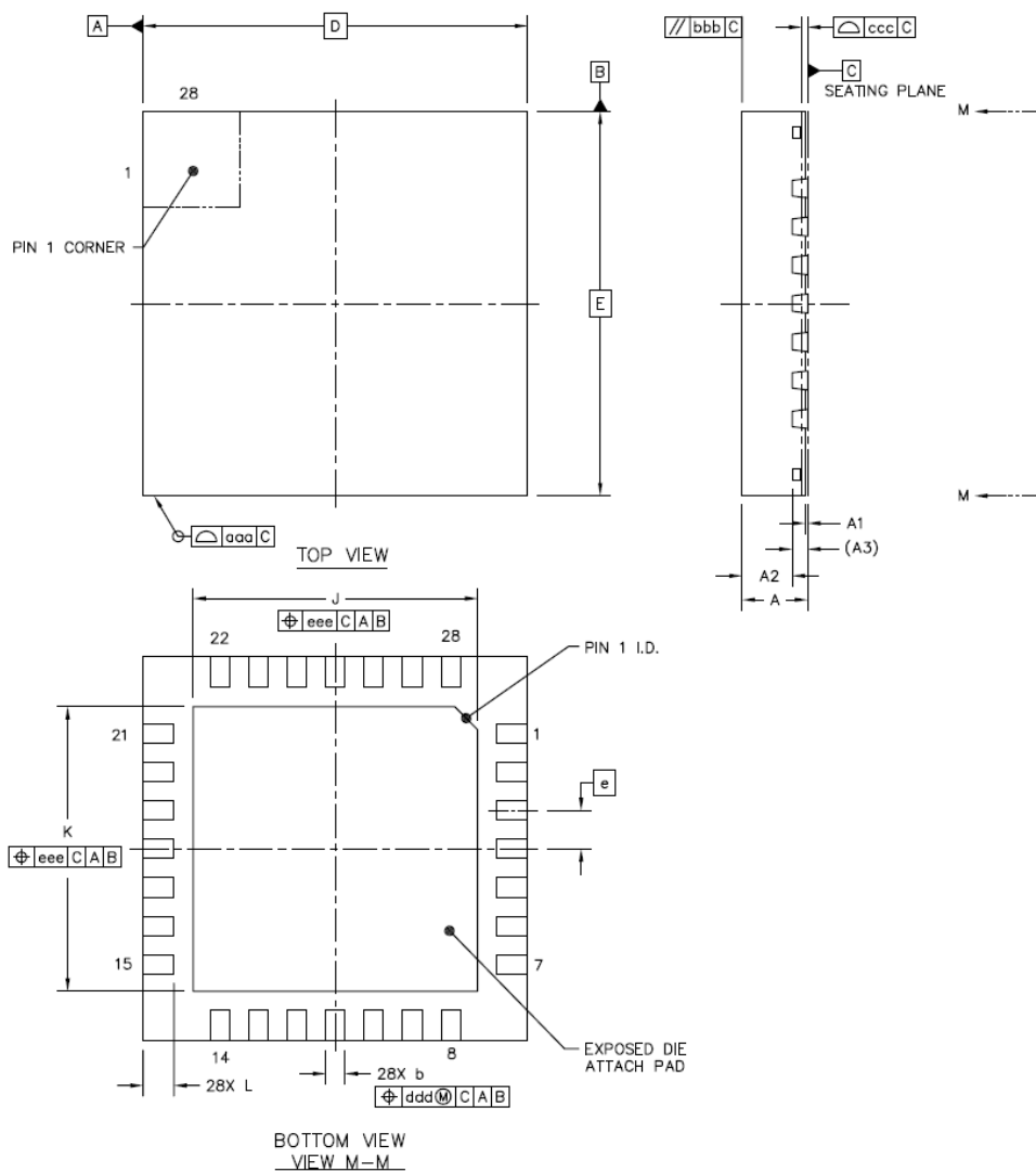
Figure 2: QFN28 (5x5mm) package outline drawings
