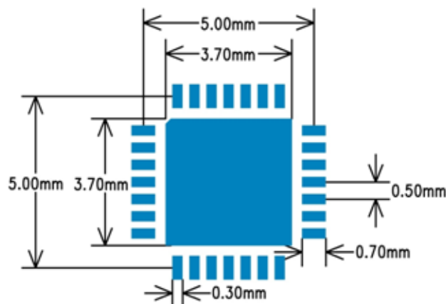
Figure 3: QFN28 (5x5mm) example land patterns (unit: mm)
