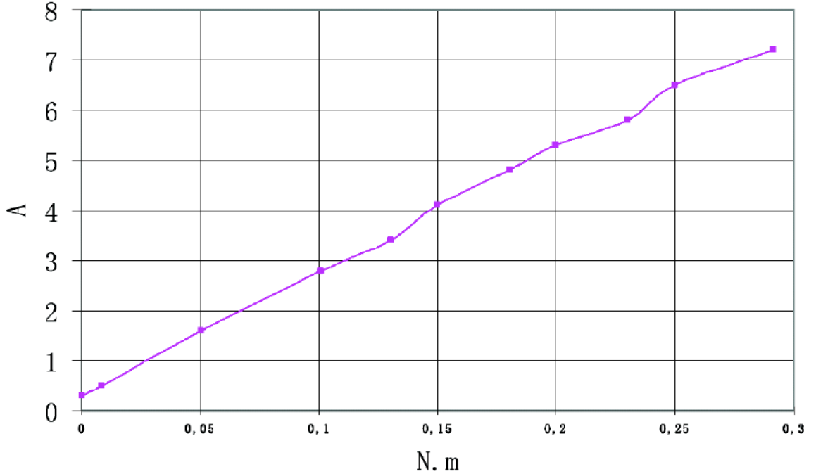
Figure 4.8: QBL4208-100-04-025 torque vs. current
